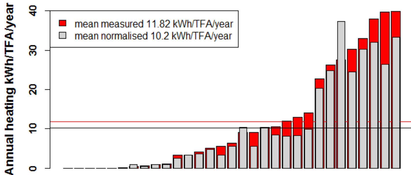
Measured and normalised annual space heating demand
