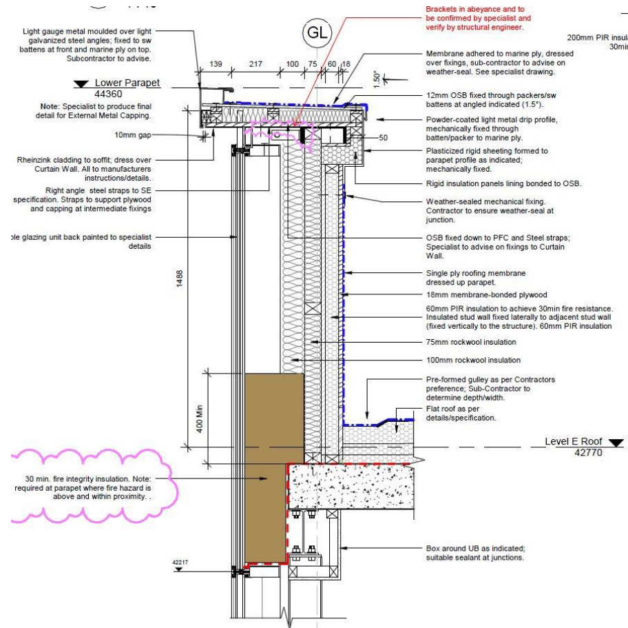
Typical Lower Parapet Detail 5 - Curtain Wall 1:10
