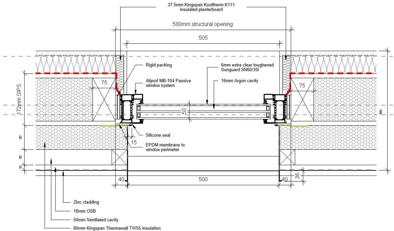
1 Typical window plan 1 : 5
