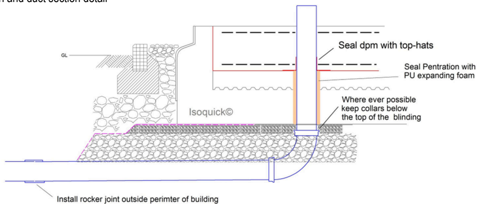
Diagram 5 - typical System installation prior to installation of DPM
