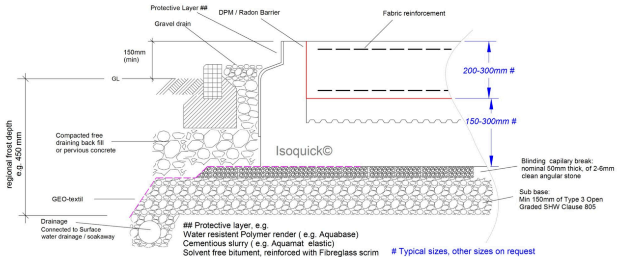
Diagram 4 - typical drain and duct section detail
